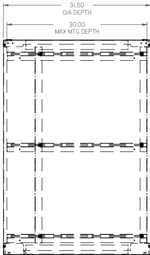
L.S. VIEW
