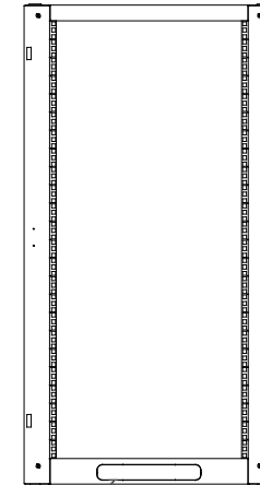
REAR VIEW
